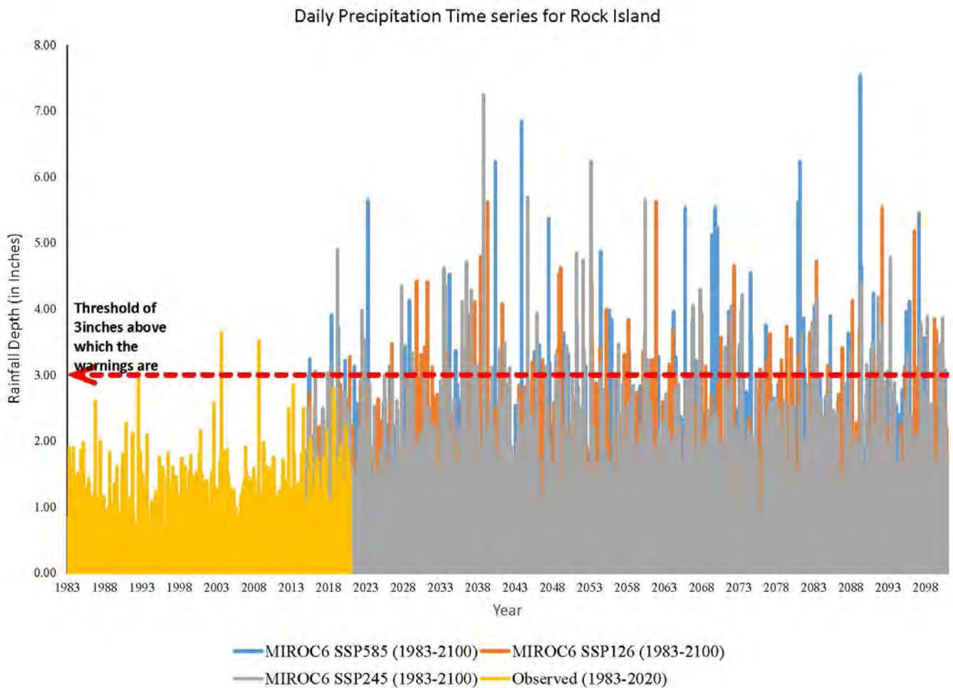
Figure 3. Trend of daily precipitation for Rock Island: low emission scenarios (SSP126; orange); intermediate emissions scenarios (SSP245; gray); very high emission scenarios (SSP585; blue). The values above the threshold are critical and are considered as warnings for floods in flood model development. The Rock Island region will also be impacted by upstream regions in the Quad Cities. The cumulative impact is further shown in flood model outputs.
